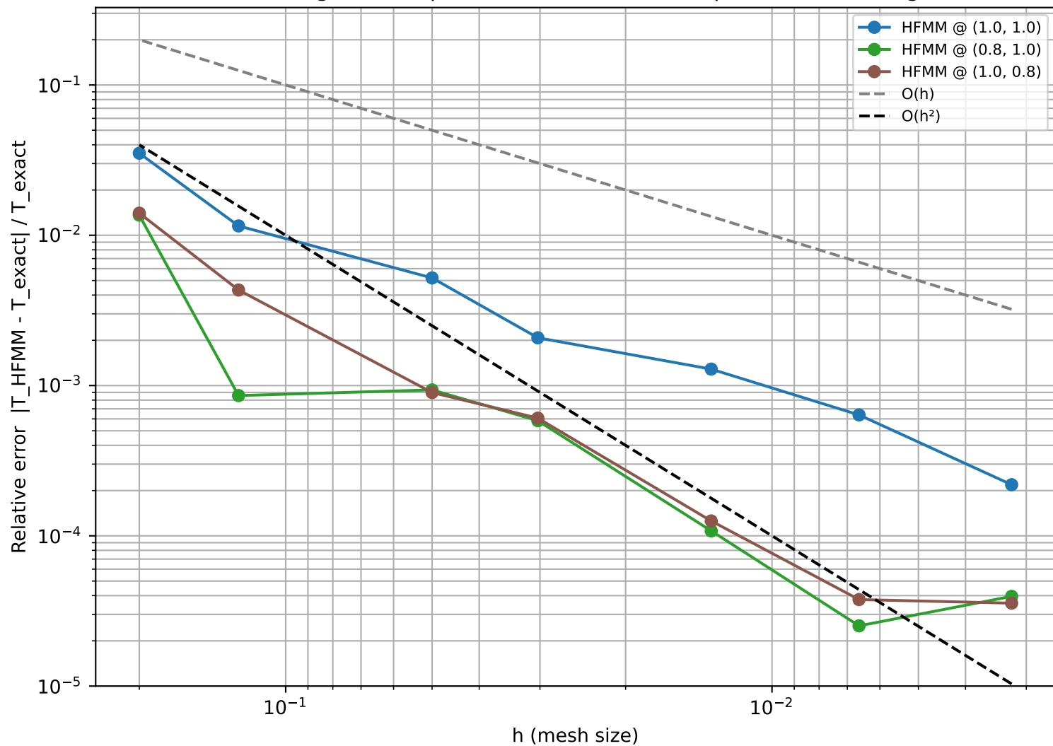
FMM Convergence - Square with Hole — HFMM pointwise convergence
